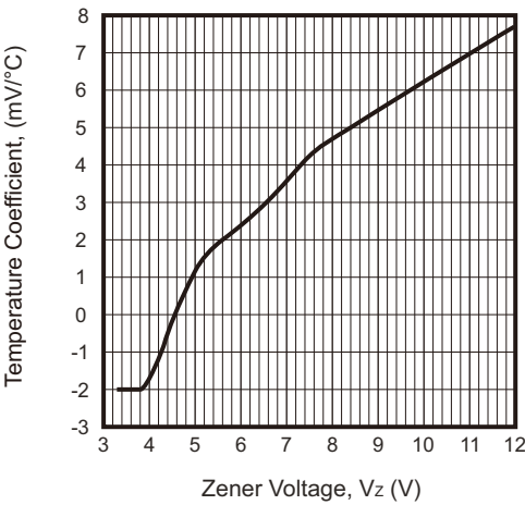
Fig.1 - Temperature Coefficient
