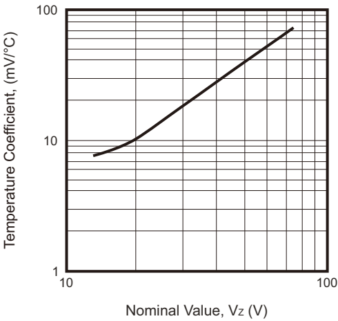
Fig.2 - Temperature Coefficient
